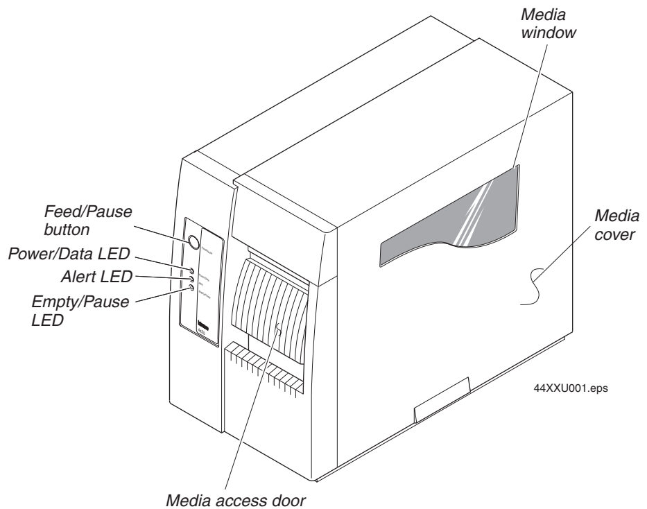
4420 and 4440 front view: This illustration shows the 4420 and 4440 features on the front of the printers.
